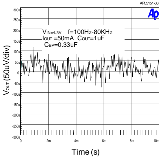
Output Noise
