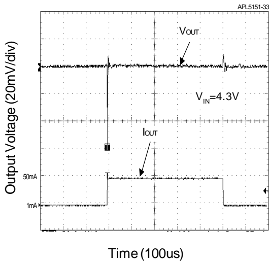
Load-Transient Response
